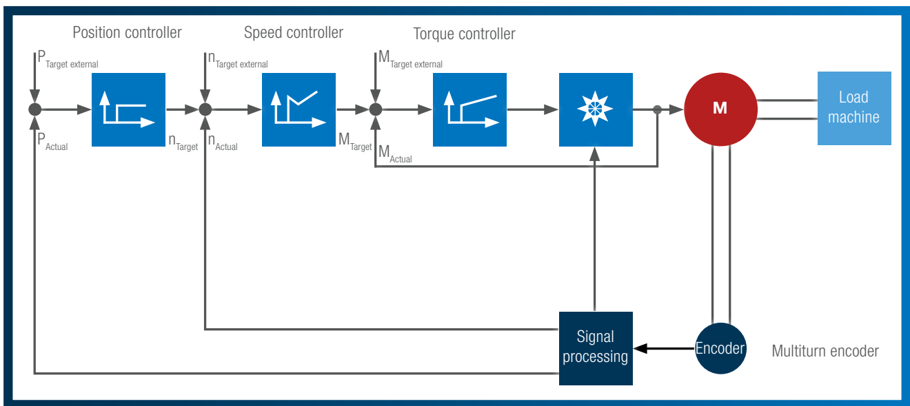
Figure: Cascaded control module
