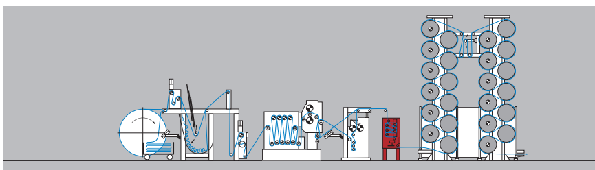
ELSTRAIGHT HD straightening system in a denim production system
