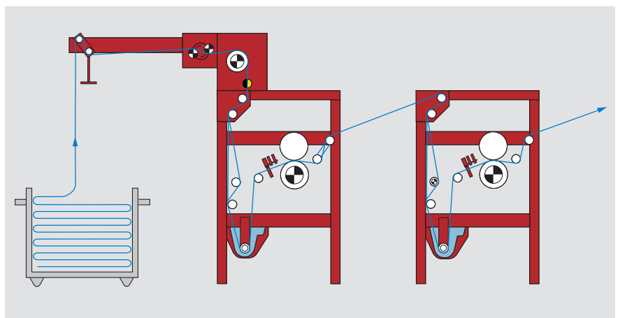
Passage of the web through the OPEN WIDTH SQUEEZING AND IMPREGNATION PADDER
