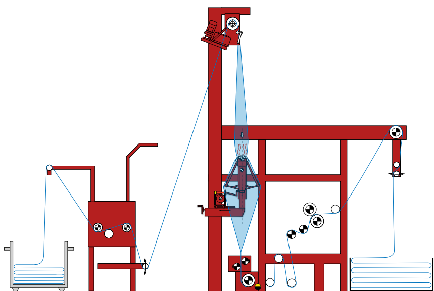
Rope opening line for wet fabrics
