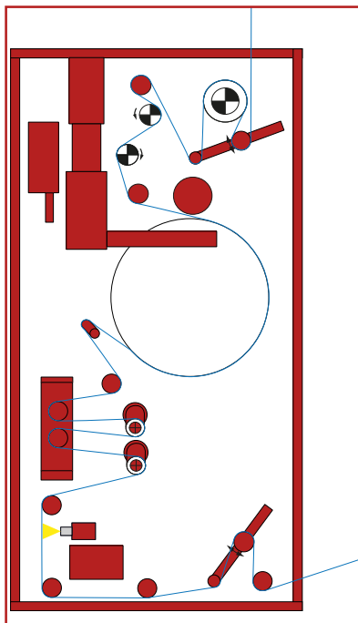
Passage of the web through the ELSTRAIGHT Combi
