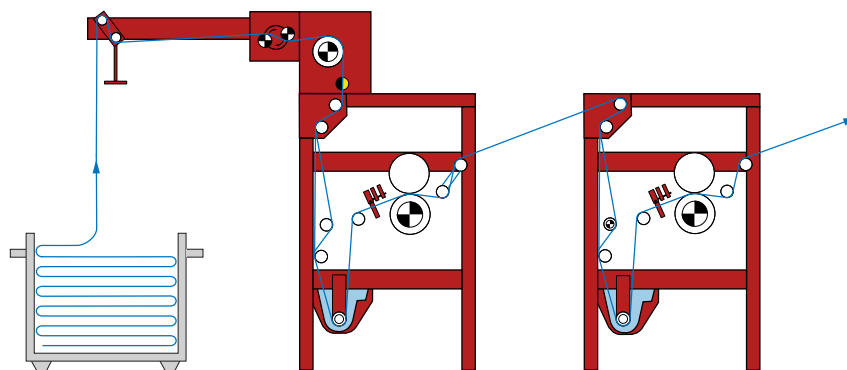
Passage of the web through the OPEN WIDTH SQUEEZING AND IMPREGNATION PADER
