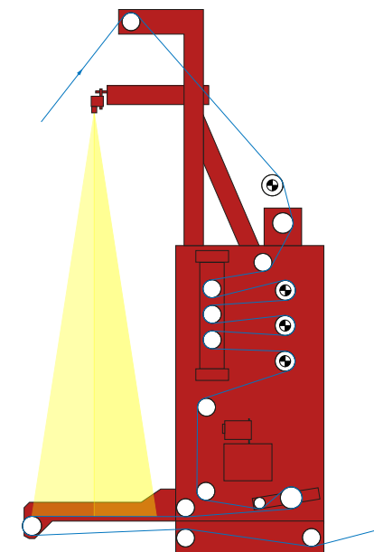
Passage of the web through ELPATTERN
