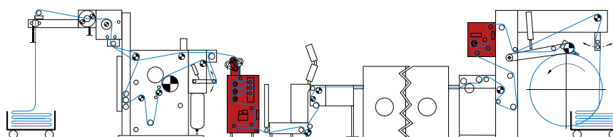
ELSTRAIGHT Mini straightening system at the outfeed of a stenter
