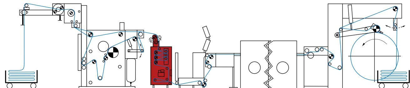
ELSTRAIGHT straightening system in the infeed of the stenter
