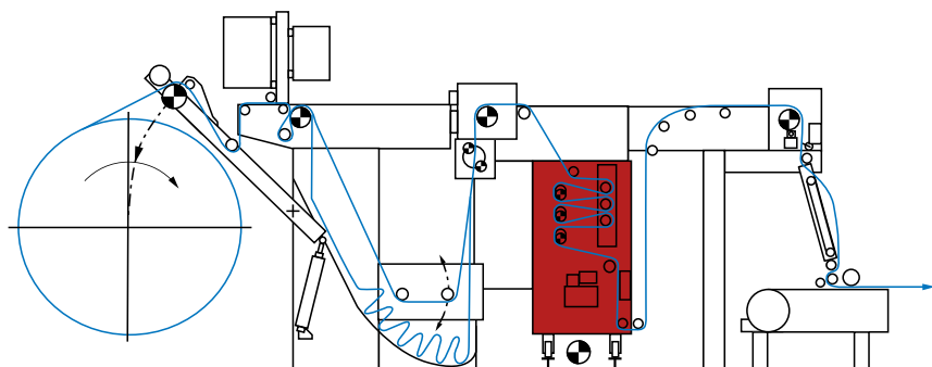
ELSTRAIGHT straightening system in the infeed of the printing machine
