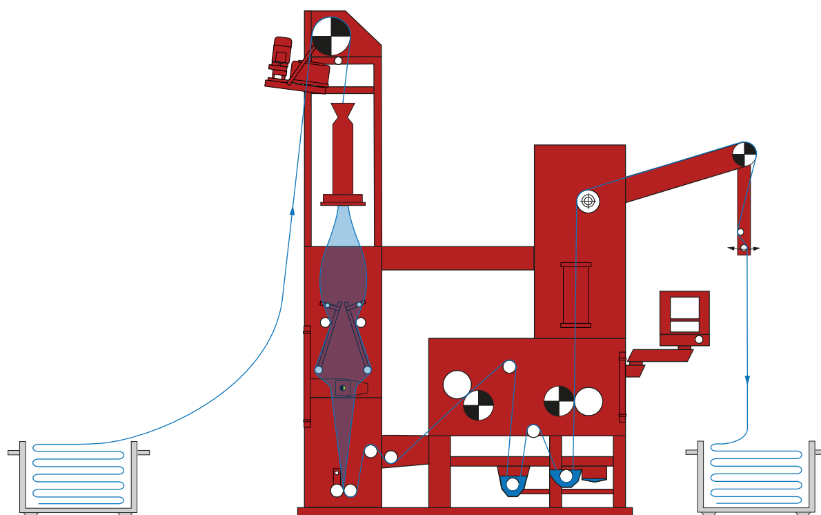
Passage of the web through the ELSTRETCH
