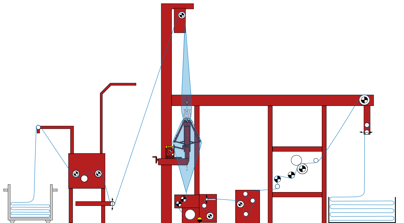
Rope opening for wet fabrics line with anti-pilling device
